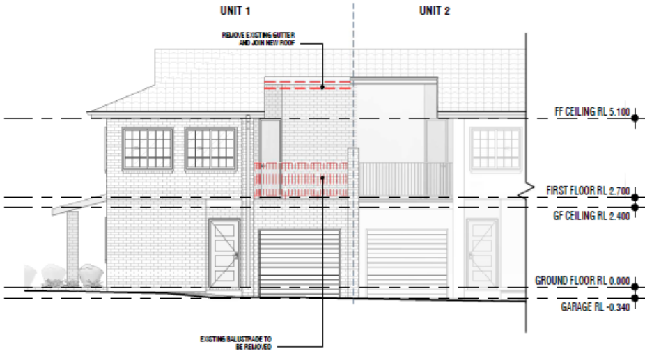
1 | FRONT ELEVATION - EXISTING
