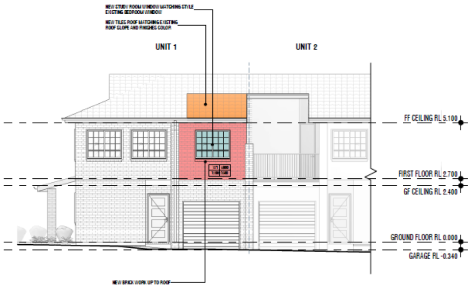
2 | FRONT ELEVATION - PROPOSED
